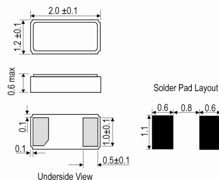
Outline (mm)
