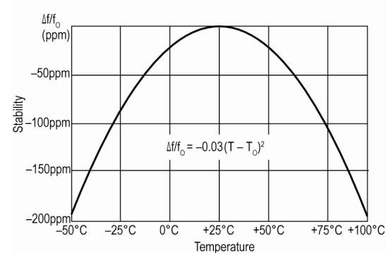
Typical Frequency Stability Characteristics
